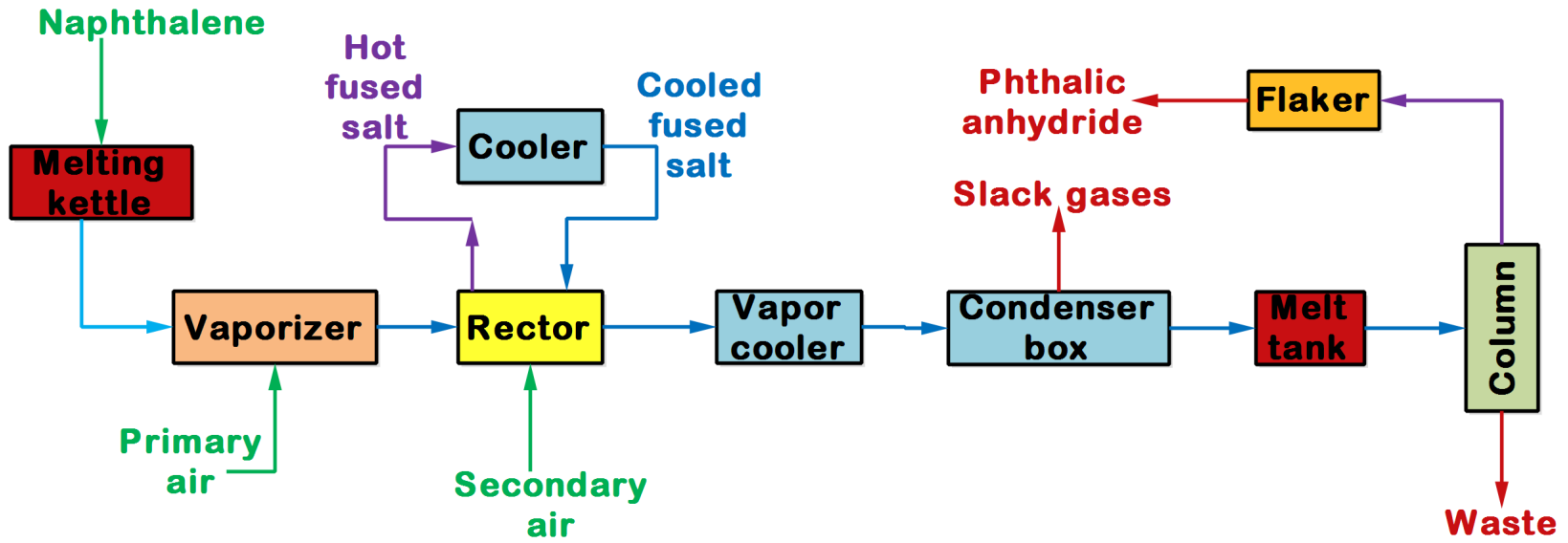
Figure: Manufacture of phthalic anhydride from naphthalene
